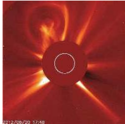
Massive 'light bulb' solar flare
